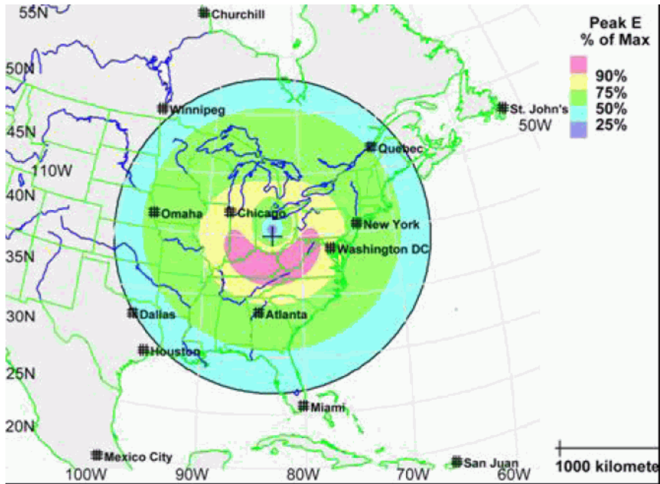
Figure 2. Illustrative EMP Effects – Fast Pulse
